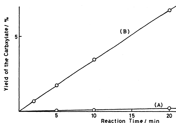
Fig. 6. The time courses of the carboxylation. (A) in the case of using CO 2 adduct with DBU, (B) in the case of using CO 2 dissolved in DMSO.
