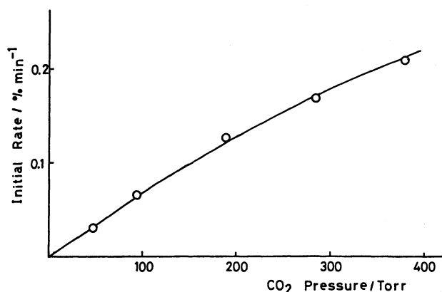
Fig. 5. The relationship between the initial rate of the carboxylation and CO 2 pressure.
